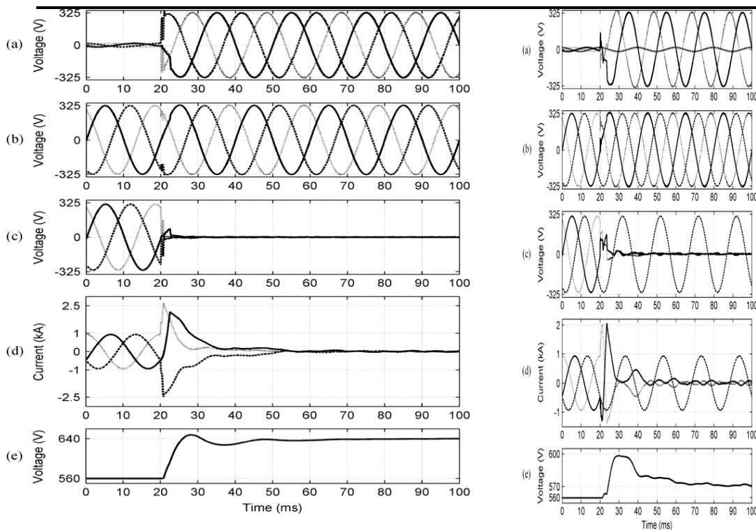
Fig.4. (a)Injectedvoltages.(b)Sourcevoltages.(c)Loadvoltages.(d)Linecurrents.(e)DC-linkvoltage, during the three- phase downstream fault.
