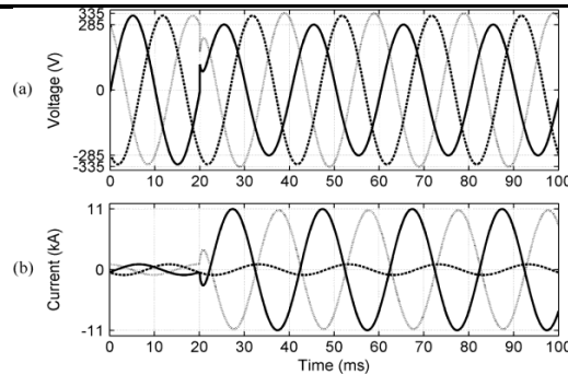
Fig.5.(a)Voltage sag,(b)Fault currents, during downstream phase-to-phase fault when the DVR is inactive(bypassed).
